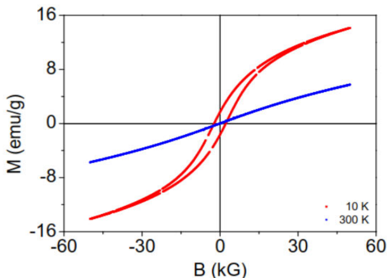
Fig. 7: M-B loops for 2 nm two lines ferrihydrite particles at two different temperatures.
