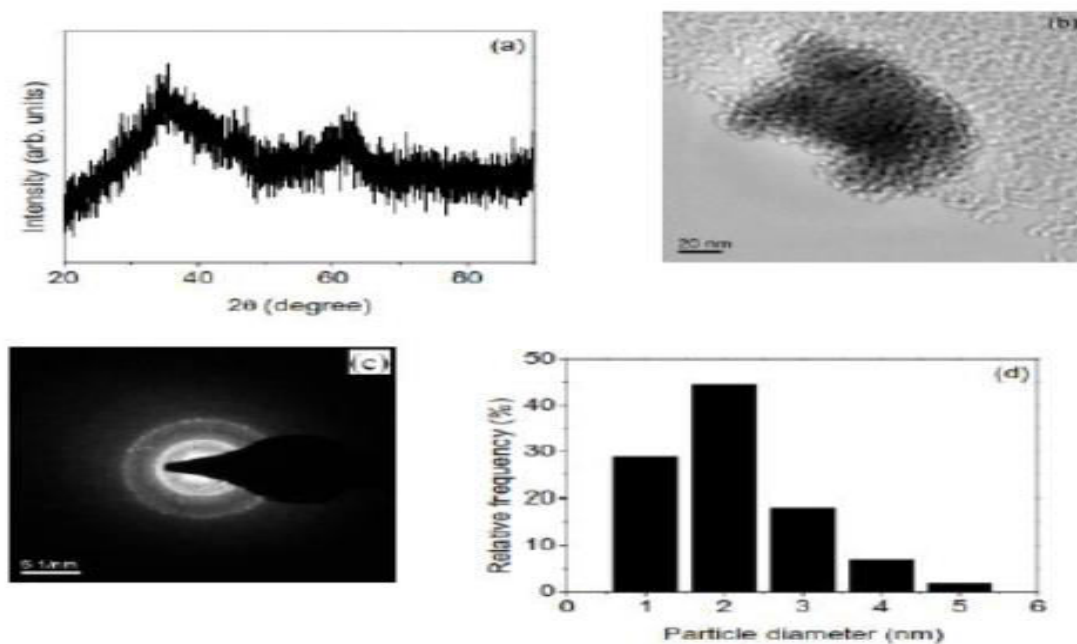
Fig. 3: (a) Room temperature x-ray diffraction pattern of the sample, (b) transmission electron micrograph of the sample, (c) selected area electron diffraction pattern and (d) a histogram of the distribution of particle size. Figure 3 (d) shows statistical distribution of particle size. This distribution is based on size measurement of 160 particles. It is found to peak at 2 nm.
