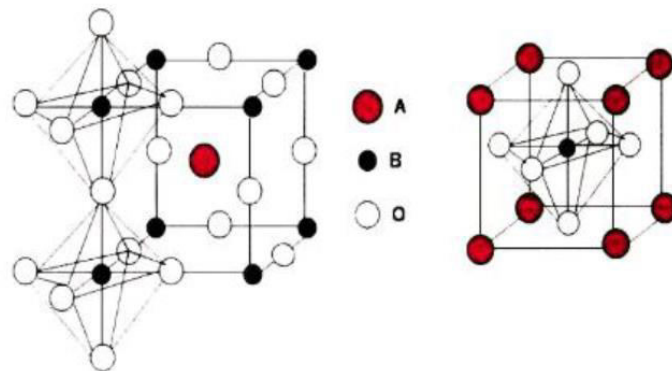
Figure 2: Structural features of an ideal perovskite, ABO 3 .
