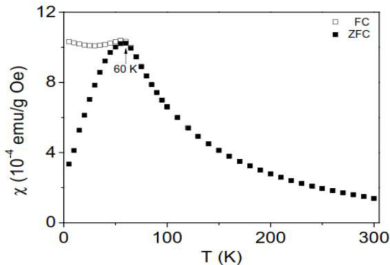
Fig. 6: ZFC (solid symbol) and FC (open symbol) susceptibility \chi as a function of temperature T for 2 nm ferrihydrite particles in 250 G applied magnetic field.
