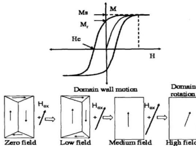
Figure 1: Basic magnetization process in ferromagnetic materials
