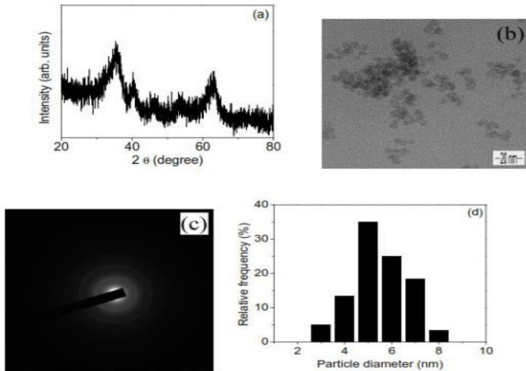
Fig. 8: (a) Room temperature x-ray diffraction pattern of the sample, (b) transmission electron micrograph of the sample, (c) selected area electron diffraction pattern and (d) a histogram of the distribution of particle size.
